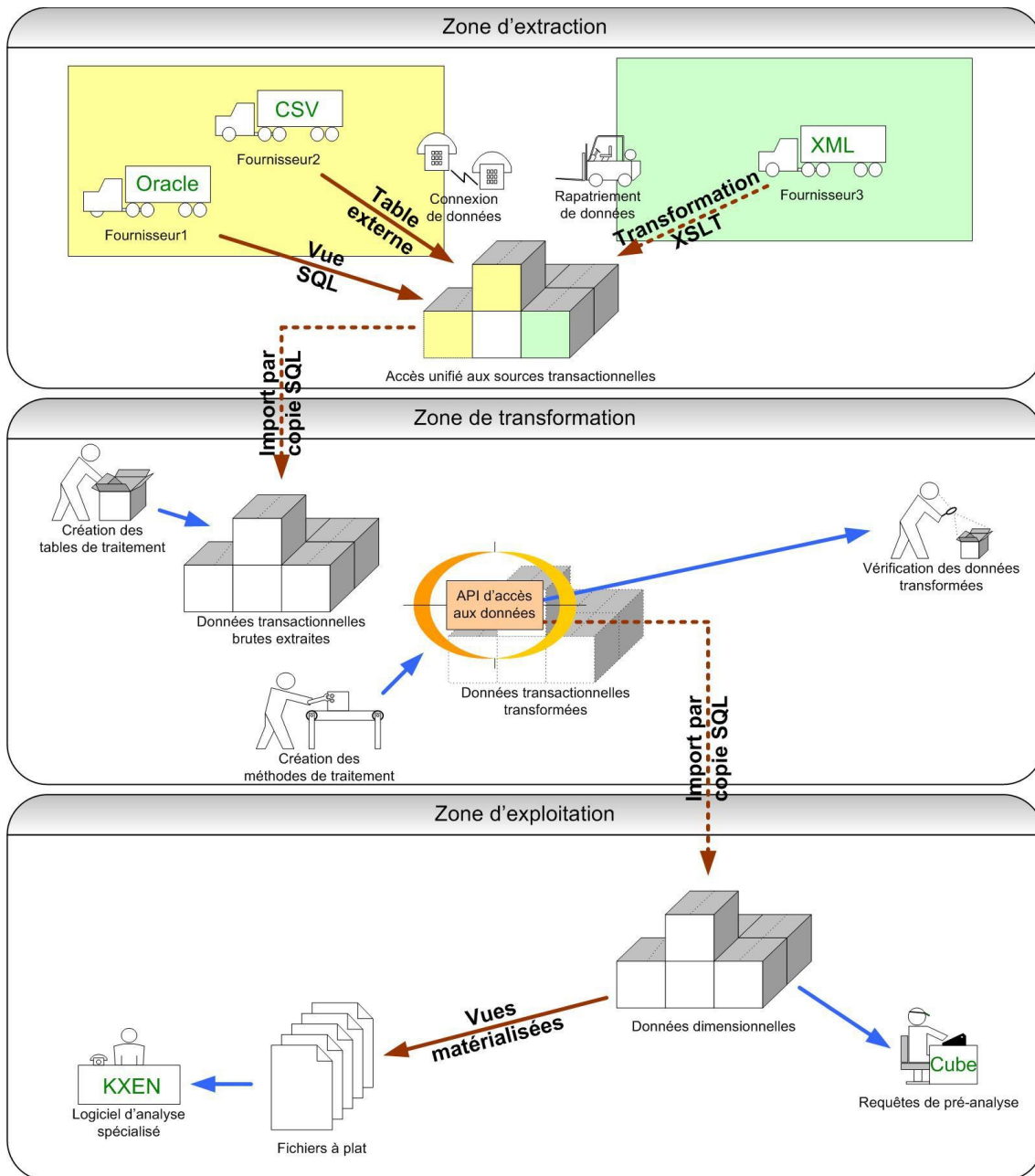
Image 1 Processus ETL
